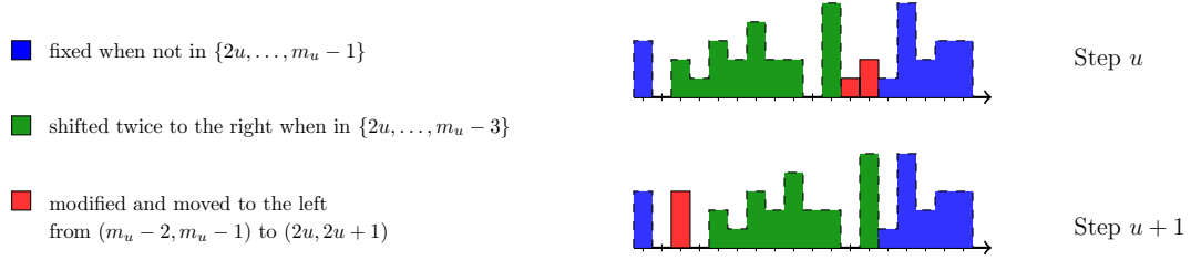
FIGURE 6. Effects of \Gamma on the multiplicity sequence from step u to step u+1 .
