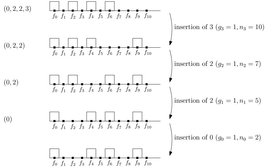
FIGURE 2. The map \Lambda in terms of frequencies.
