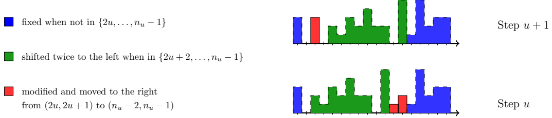
FIGURE 5. Effects of \Lambda on the multiplicity sequence from step u + 1 to step u .
