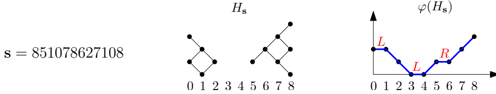
Fig. 3: An alternating word \mathbf{s} with corresponding heap H_{\mathbf{s}} , and its encoding by a walk.
