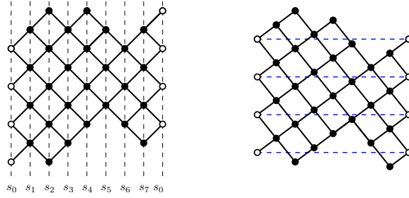
FIGURE 1. Representation of a FC heap of type \tilde{A}_7 .
