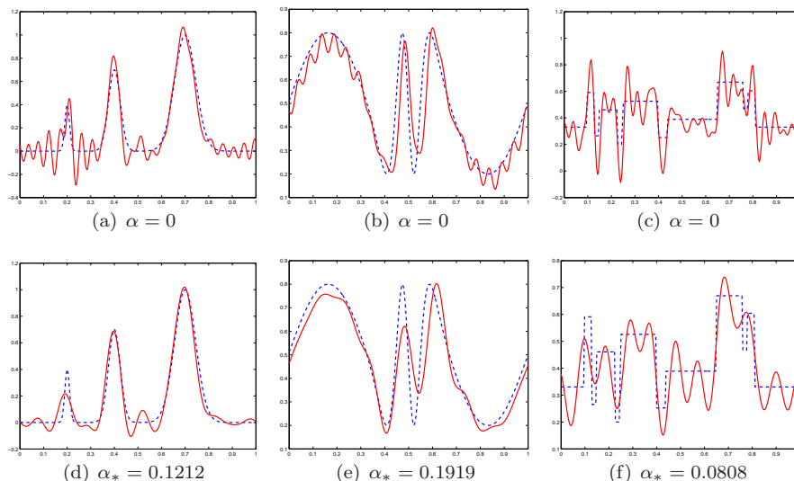
FIG 2. An example of template estimation ( n = 20 and rsnr = 7 ) with \alpha = 0 and \alpha = \alpha_* for each test function.
