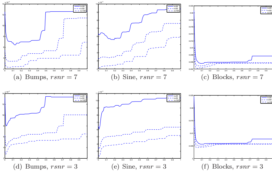
FIG 3. Empirical Mean Square Error (MSE) over M = 100 simulations as a function of \alpha \in [0, 1] for n = 20, 50, 100 and rsnr = 7, 3 for each test function: Bumps (first column), Sine (second Column), Blocks (third column).
