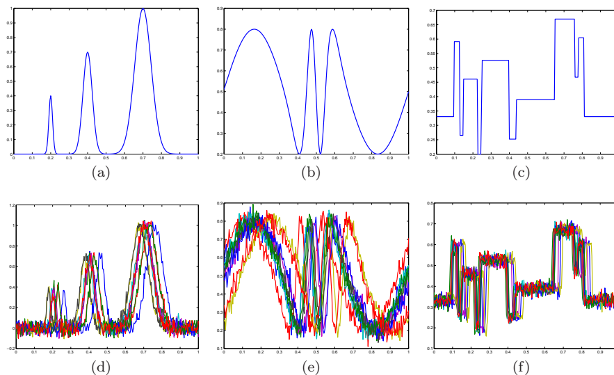
FIG 1. Test functions and an example of randomly shifted curves. First line: (a) Bumps, (b) Sine, (c) Blocks. Second line: sample of 10 curves out of n = 20 for each test function.
