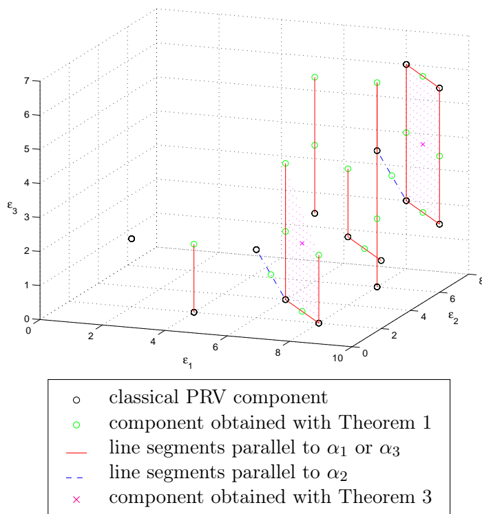
Figure 2: some weights of V_{\mathrm{Sp}_6}(2, 0, 4) \otimes V_{\mathrm{Sp}_6}(2, 0, 2)
