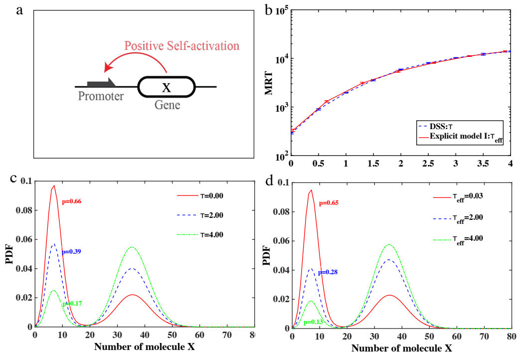
FIG. 1. a) A schematic diagram of self-activation circuit. b) Mean residence time calculated with DSS and explicit model I. c) Equilibrium distribution calculated with DSS. d) Equilibrium distribution calculated by explicit model I. p is the proportion occupied by low number state. For all plots parameter values \alpha = 5, c = 19, \gamma = \ln(2) and b = 10 are used. MRT and PDF stand for mean residence time and probability density function respectively.
