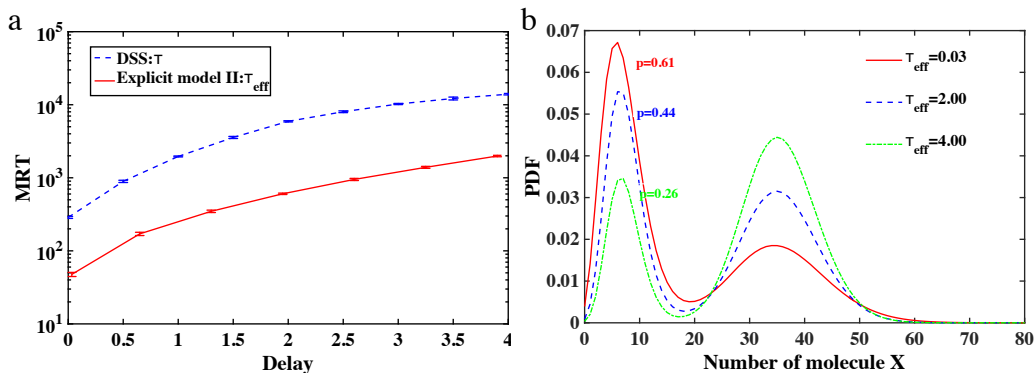
FIG. 2. a) Mean residence time calculated by the DSS and by explicit model II. b) Equilibrium distribution calculated by explicit model II. p is the proportion occupied by low number state. All parameters are the same as in Fig 1.
