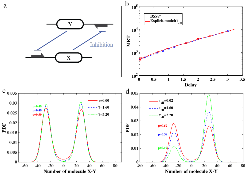
FIG. 4. a) A schematic diagram of toggle-switch circuit. b) Mean residence time of X < Y state calculated by DSSs and the explicit model. c) Equilibrium distribution calculated by DSSs. d) Equilibrium distribution calculated by explicit model. p is the proportion occupied by the X < Y number state. \beta = 21.9, k = 6.8, \gamma = \ln(2)
