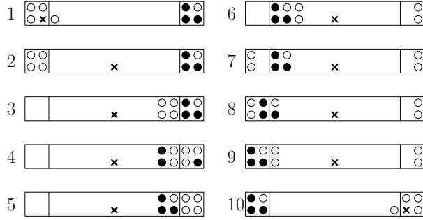
FIGURE 4. An example of the main steps in the construction of the path from \eta (in line 1) to \tau_y(\eta^{0y, \square}) (in line 10) when y = (L + 2)e_1 . Only the liaison tube is represented. From line 1 to 2 we use Lemma 5.5; line 2 to 3: Lemmata 5.6 and 5.4 twice; line 3 to 4: Lemmata 5.6 and 5.4; line 4 to 5: Lemmata 5.7, 5.6; line 5 to 6: Lemmata 5.6, 5.4; line 6 to 7: Lemmata 5.4, 5.6, 5.7; line 7 to 8: Lemmata 5.6, 5.4; line 8 to 9: Lemmata 5.7, 5.6; from 9 to 10, Lemmata 5.4, 5.6, 5.5.
