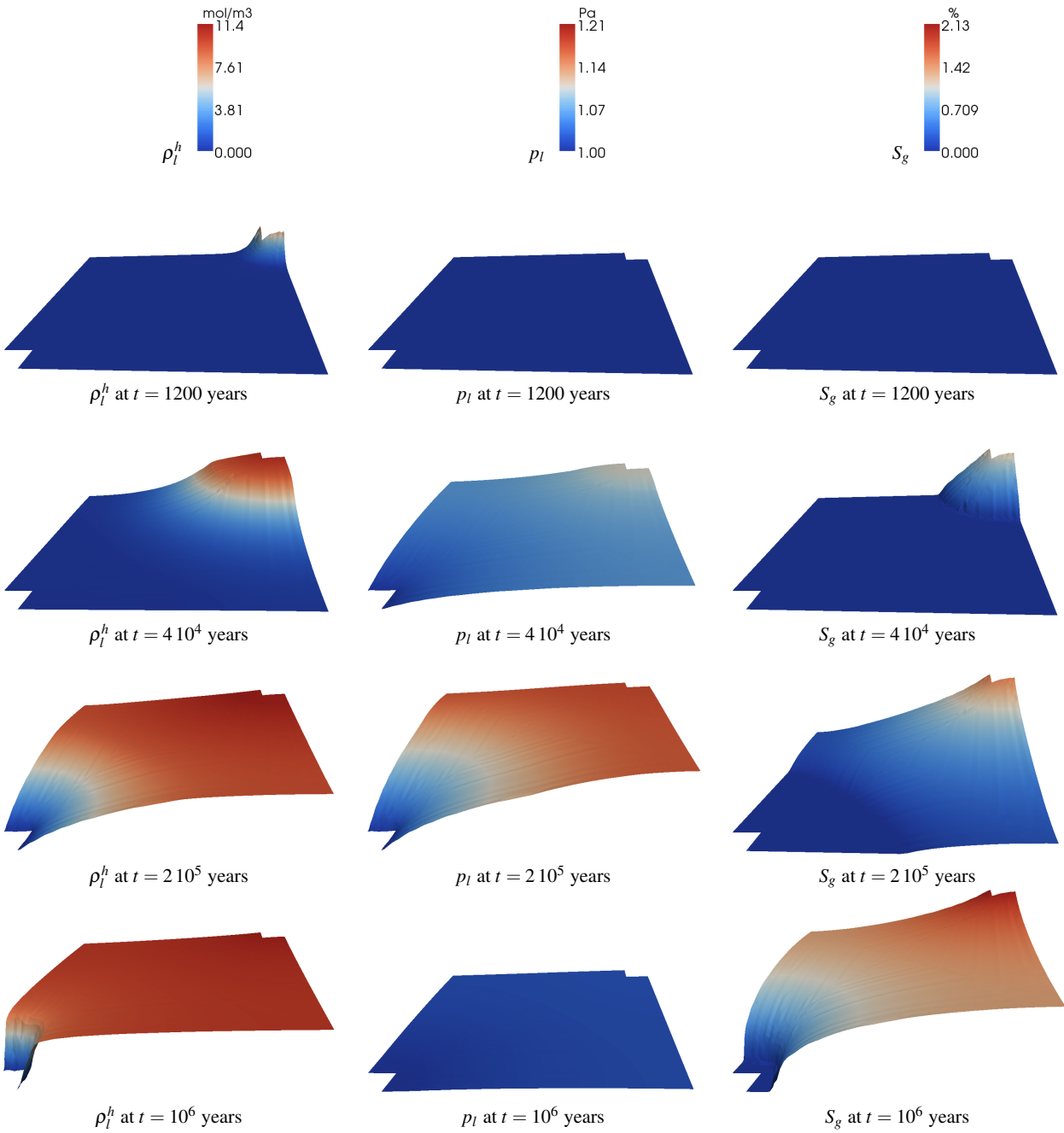
Fig. 5 Numerical Test case number 1: Evolution of \rho_l^h , the hydrogen density in the liquid phase; p_l the liquid phase pressure; and S_g the gas saturation; at times t = 1200, 4 \cdot 10^4, 2 \cdot 10^5 and 10^6 years (from the top to the bottom).
