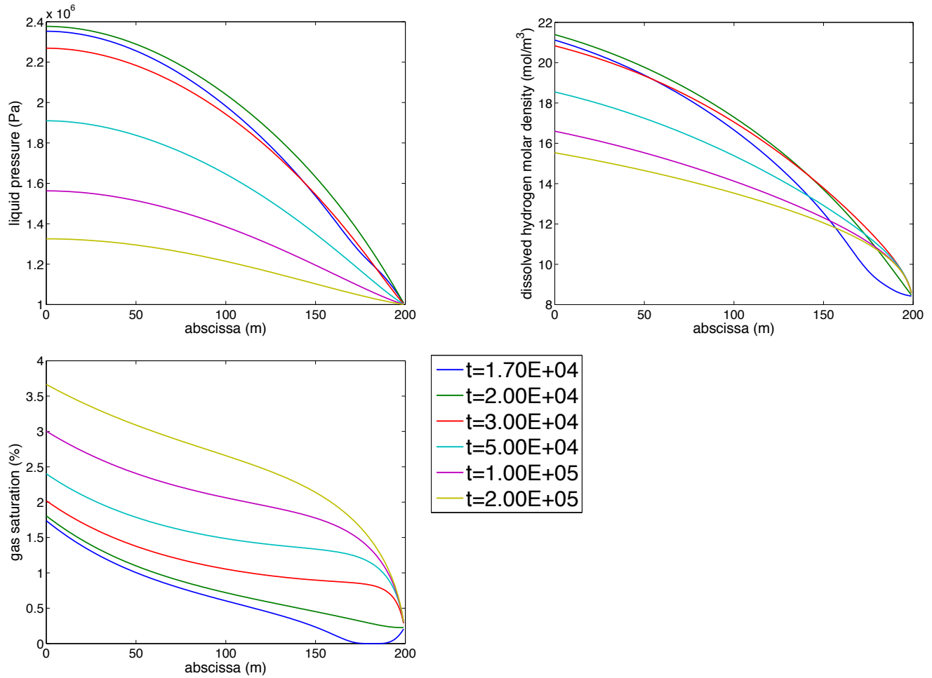
Fig. 7 Test case number 2; L_x = L_2 = 200 m. Time evolution, in years, of c_l^h the dissolved hydrogen molar density (top right), p_l (top left) and S_g (bottom) profiles, during the last period of time.
