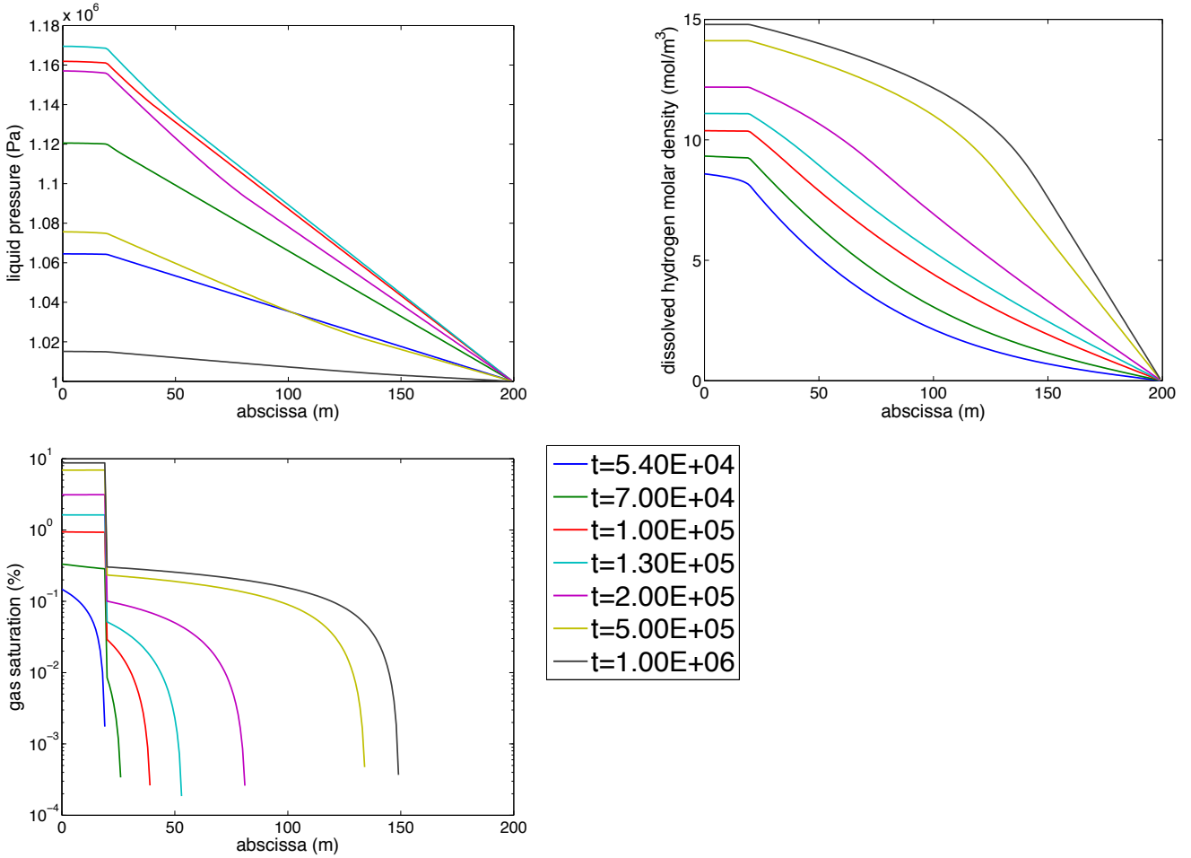
Fig. 10 Test case number 3; L_x = 200 m, L_1 = 20 m. Time evolution, in years, of c_i^h the dissolved hydrogen molar density (top right), p_l (top left) and S_g (bottom) profiles, during the last period of time.
