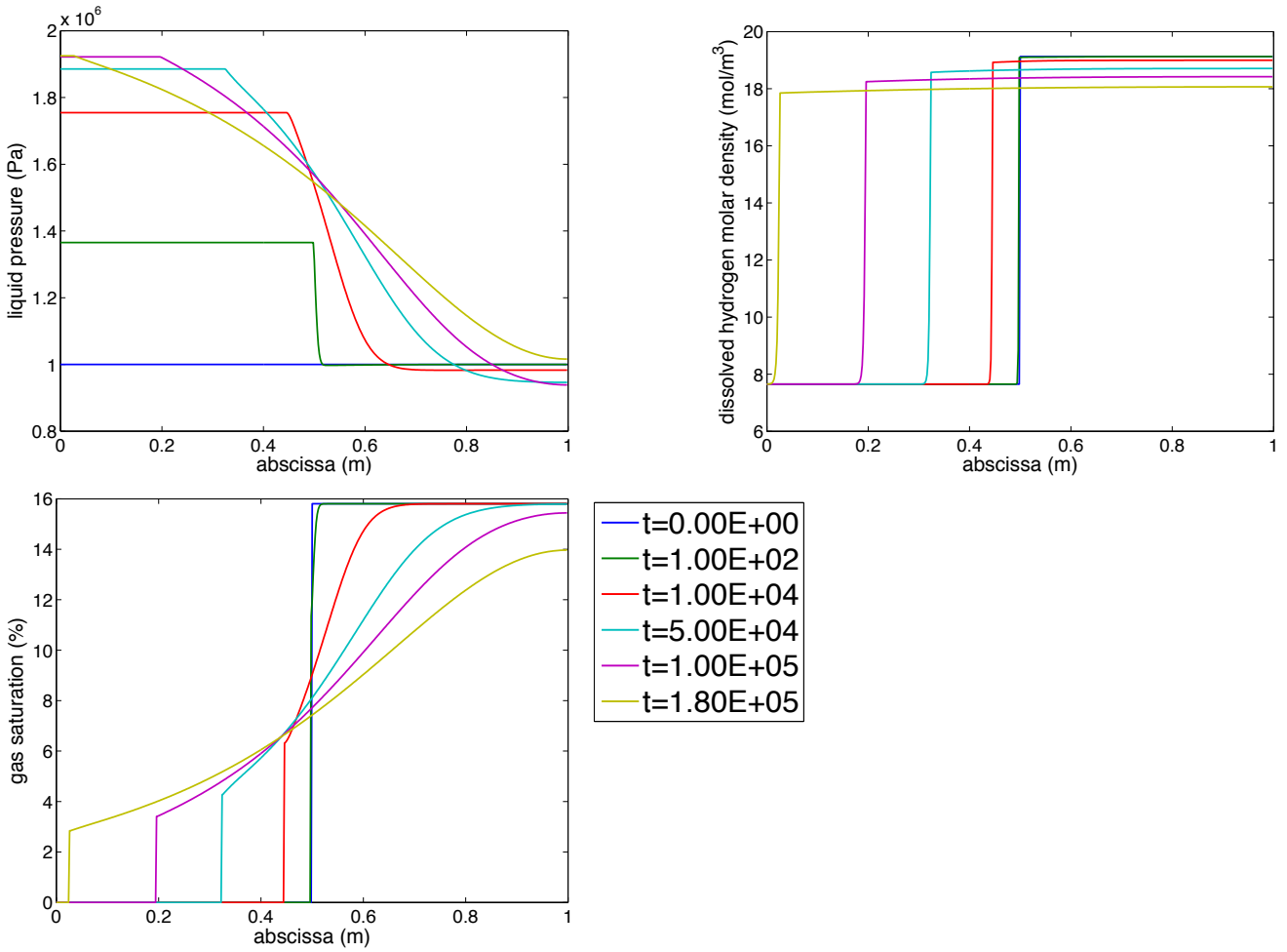
Fig. 11 Numerical test case number 4, L_x = 1 m, L_1 = 0.5 m: Time evolution, in seconds, of c_l^h the dissolved hydrogen molar density (top right), p_l (top left) and S_g (bottom) profiles, during the first period of time.
