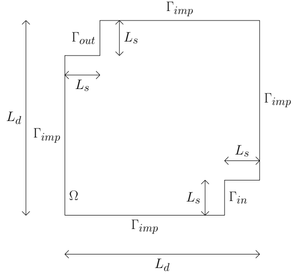
Fig. 3 Test case number 1: Geometry of the 2-D porous domain, \Omega .
