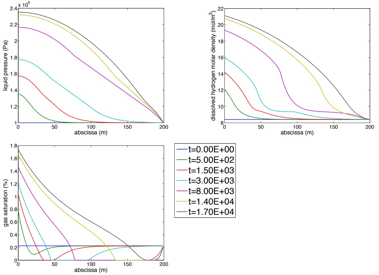
Fig. 6 Test case number 2; L_x = L_2 = 200 m. Time evolution, in years, of c_l^h the dissolved hydrogen molar density (top right), p_l (top left) and S_g (bottom) profiles, during the first period of time.
