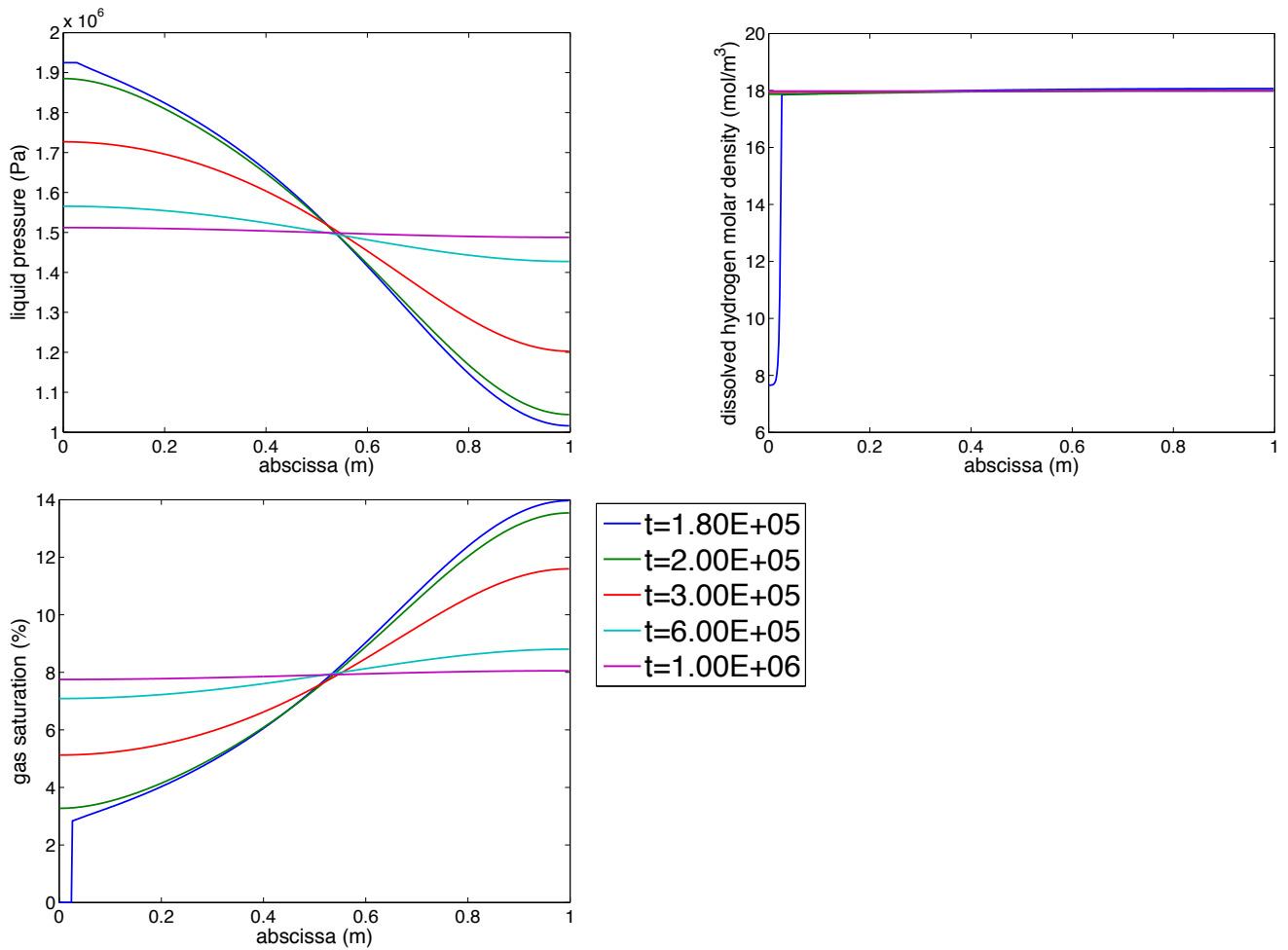
Fig. 12 Numerical test case number 4, L_x = 1 m, L_1 = 0.5 m: Time evolution, in seconds, of c_l^h the dissolved hydrogen molar density (top right), p_l (top left) and S_g (bottom) profiles, during the last period of time.
