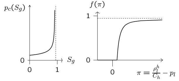
Fig. 2 Capillary pressure curve, p_c = p_g - p_l , and inverse function
