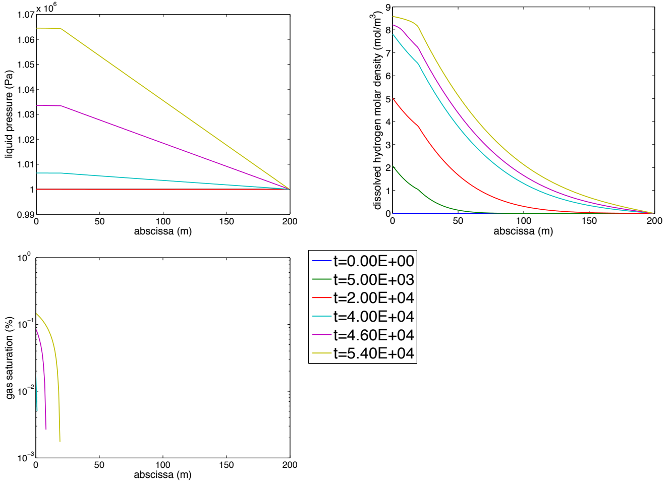
Fig. 9 Test case number 3; L_x = 200 m, L_1 = 20 m. Time evolution, in years, of c_l^h the dissolved hydrogen molar density (top right), p_l (top left) and S_g (bottom) profiles, during the first period of time.
