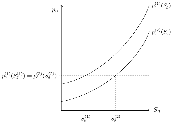
Fig. 8 Saturation discontinuity at the interface of two materials with different capillary pressure curves; test case number 3.
