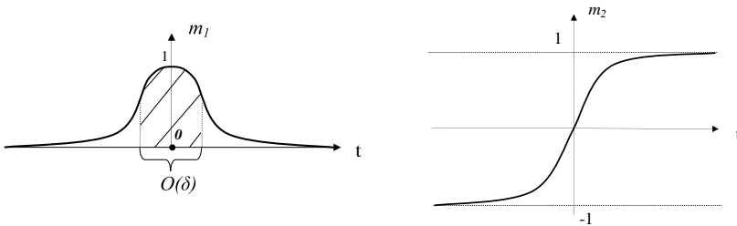
Fig. 15. First and second component of a 180° Néel wall.
