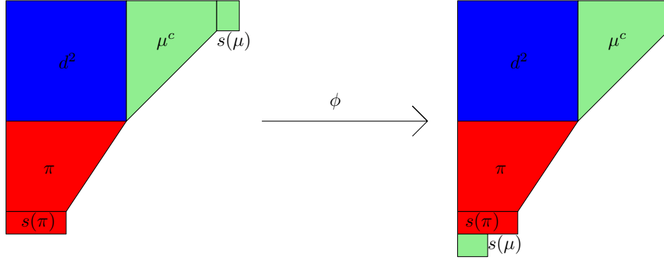
FIGURE 1. The case 2 of the involution \phi
