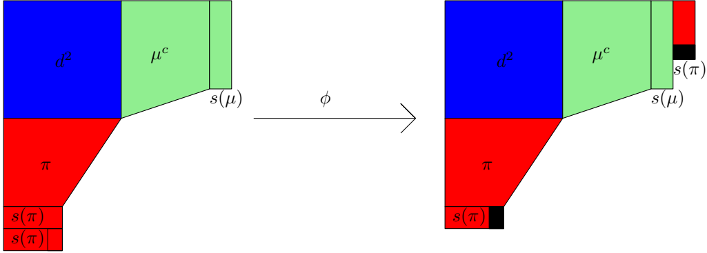
FIGURE 2. The case 3.1 of the involution \phi
