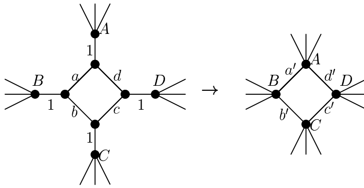
FIGURE 6. Urban Renewal, a' = \frac{c}{ac+bd} , b' = \frac{d}{ac+bd} , c' = \frac{a}{ac+bd} , d' = \frac{b}{ac+bd} .
