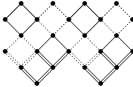
FIGURE 14. The double edges have weight \frac{2}{3} , the dotted double edges have weight \frac{1}{3} , the dotted edges have weight \frac{2}{5} and the remaining edges have weight \frac{4}{5} .
