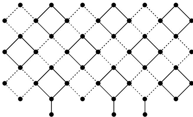
FIGURE 7. The dotted lines have weight \frac{1}{2} .
