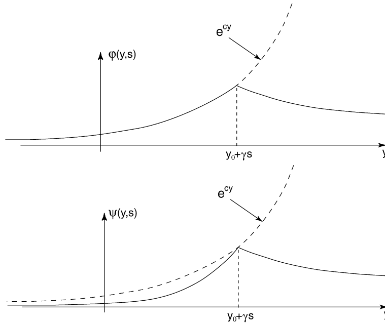
Fig. 3. Graphs of the weight functions \varphi(y, s) and \psi(y, s) .
