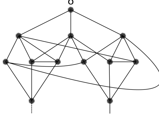
FIGURE 5.1: Example of graph which verifies Assumption 5.1.1
