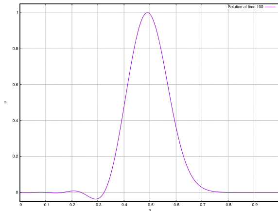
Figure 4: Solution with the Crank-Nicolson scheme ( \theta = 1/2 ) at time 100 for J = 1000
