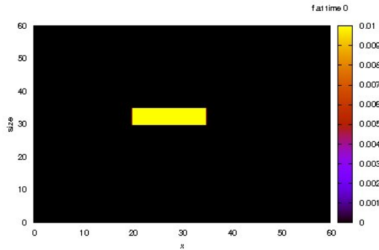
Figure 1: initial density.
