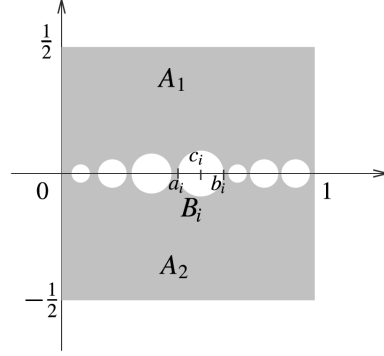
Fig. 1. An example illustrating the fact that the M -connected components of an open set do not coincide in general with the classical connected components
