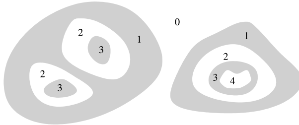
Fig. 3. The topographic function associated with the gray set E counts how many boundaries must be crossed to reach the exterior of E
