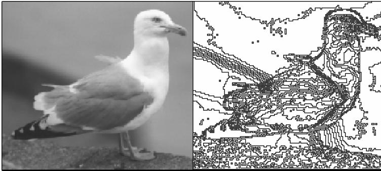
Fig. 5. An image and its partial topographic map (grey level step = 10)
