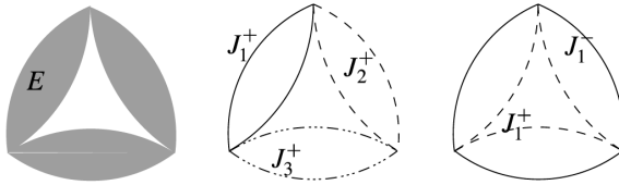
Fig. 2. The set E (in grey), its boundaries J_i^\pm and the boundaries of its complement. The last figure illustrates as well the internal and external boundaries obtained by the topographic function
