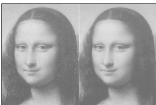
Fig. 7. An uncorrupted image and the result of the filtering by I_{10}S_{10} . This experiment illustrates the ability of Vincent's filter to preserve uncorrupted parts of an image
