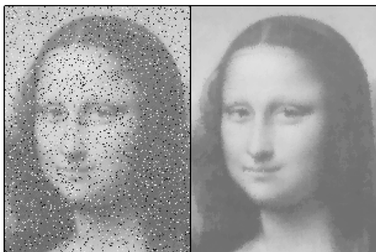
Fig. 6. An image corrupted by an impulse noise with frequency 15% and the result of the denoising performed by I_{10}S_{10}
