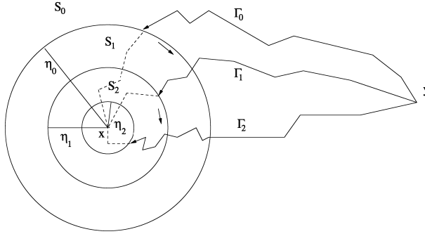
Fig. 4. Recursive construction of \Gamma near to x
