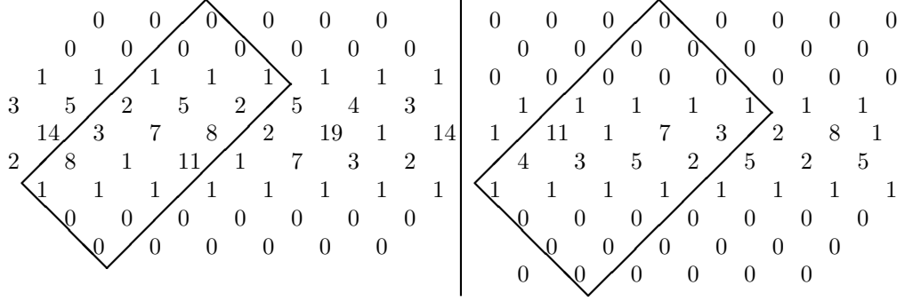
FIGURE 2. An SL_3 -frieze of width 3 (matrix A left) and its Gale dual SL_4 -frieze of width 2 (matrix A' right).
