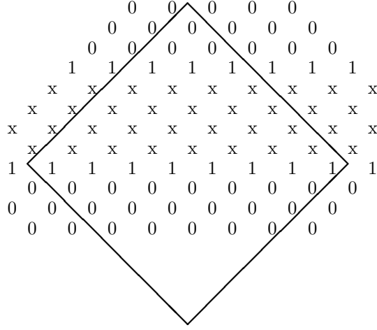
FIGURE 3. Cutting a unitriangular matrix out of a frieze.
