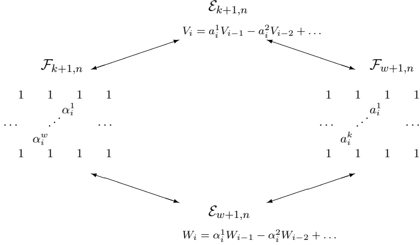
FIGURE 1. Duality between periodic difference equations, friezes of solutions and friezes of coefficients.
