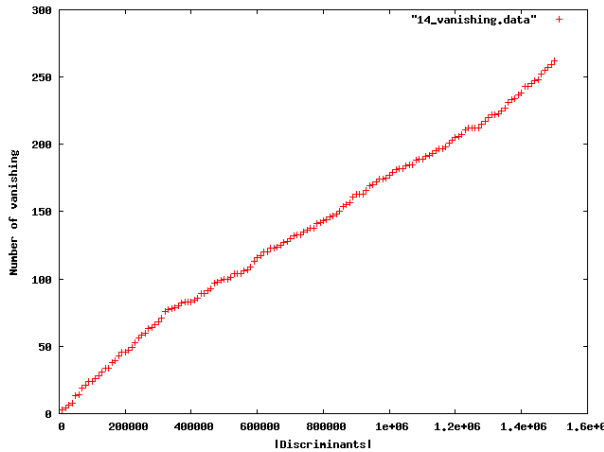
Figure 11: Number of extra-vanishing of L'(E_d, 1) for E = 14a1 .
