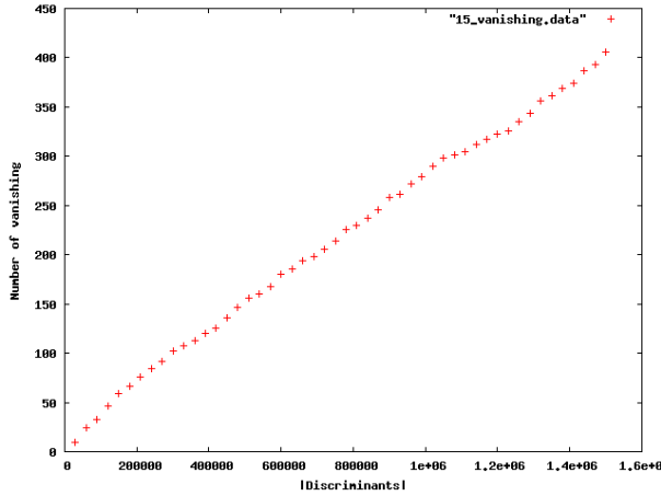
Figure 14: Number of extra-vanishing for L'(E_d, 1) for E = 15a1 .
