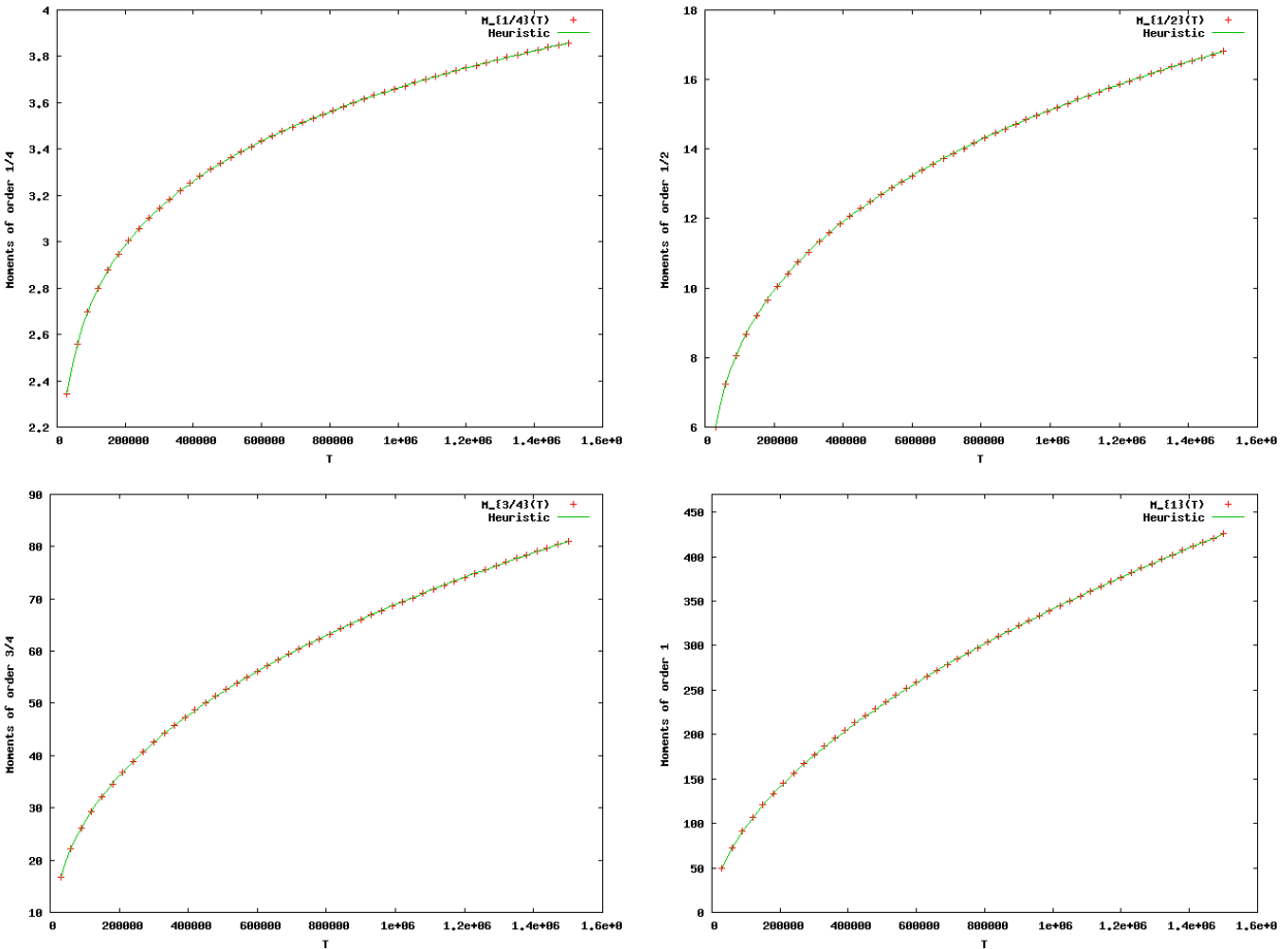
Figure 2: Moments of order \frac{1}{4} , \frac{1}{2} , \frac{3}{4} and 1 of the regulators of the twists of 11a1 and the function given by the heuristics.
