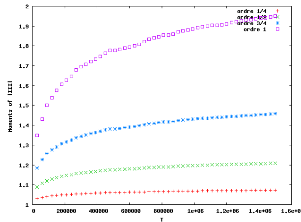
Figure 9: Moments of order \frac{1}{4} , \frac{1}{2} , \frac{3}{4} and 1 for the order of the Tate-Shafarevich groups of the twists of 17a1 . The heuristics suggest that the moments of order k < 1 tend to a constant (depending on k ) whereas the moment of order 1 should tend to infinity.
