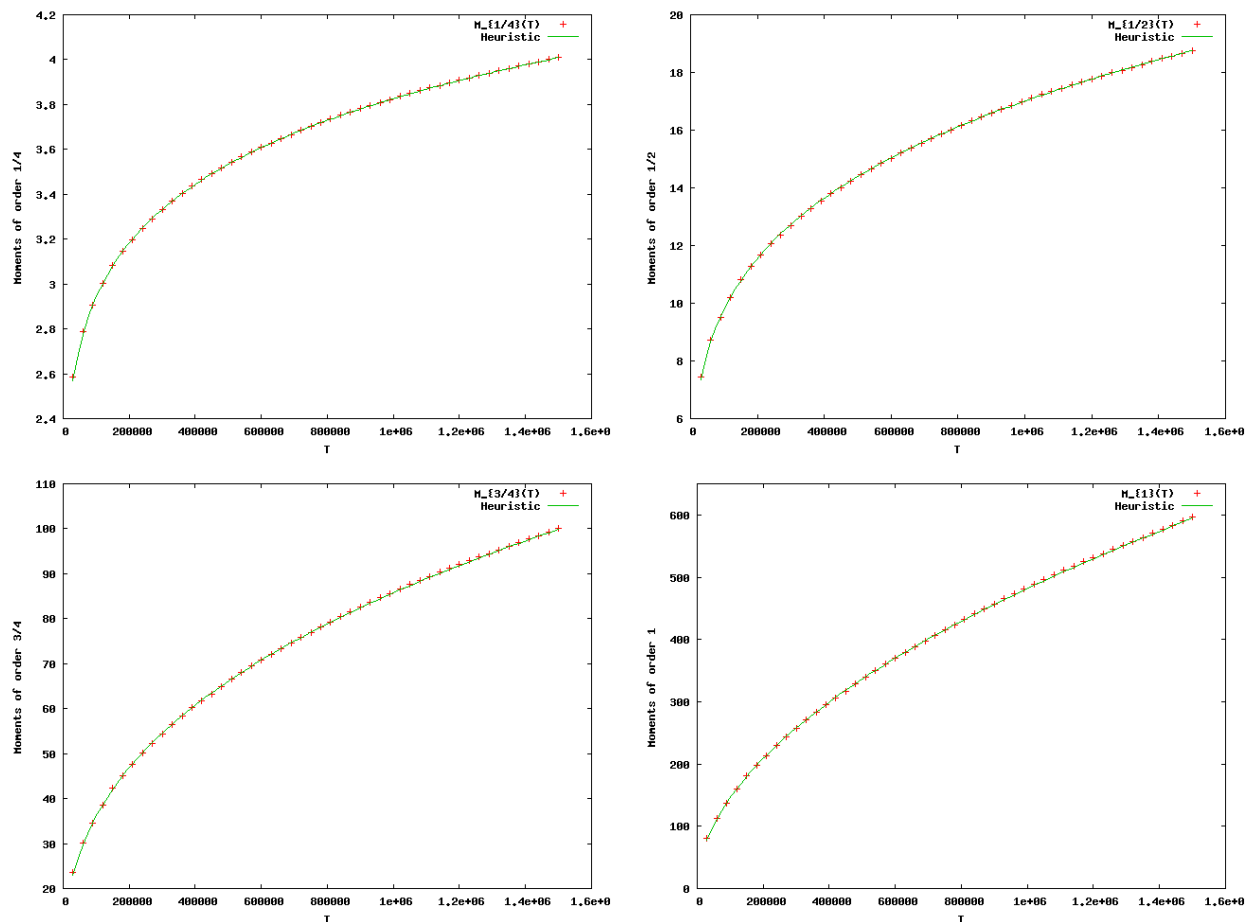
Figure 16: Moments of order \frac{1}{4} , \frac{1}{2} , \frac{3}{4} and 1 for the regulators of the twists of 15a1 and the functions given by the heuristics.
