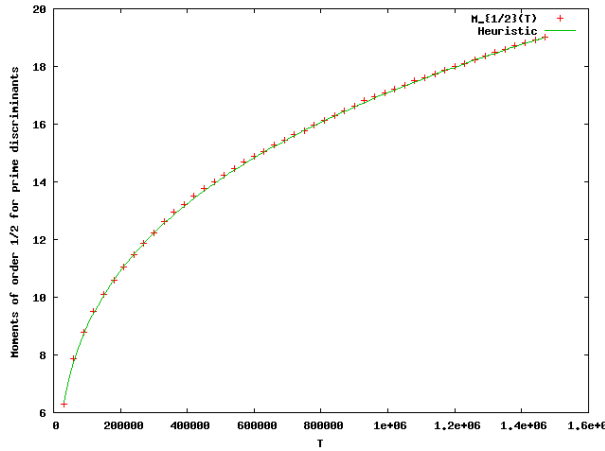
Figure 5: Moments of order \frac{1}{2} and 1 for the regulators of the twists of 11a1 by prime discriminants and the functions given by the heuristics.
