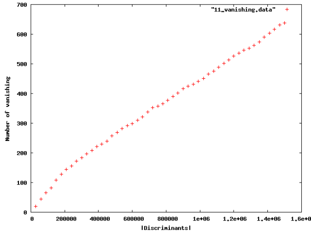
Figure 3: Number of extra-vanishing of L'(E_d, 1) for E = 11a1 .
