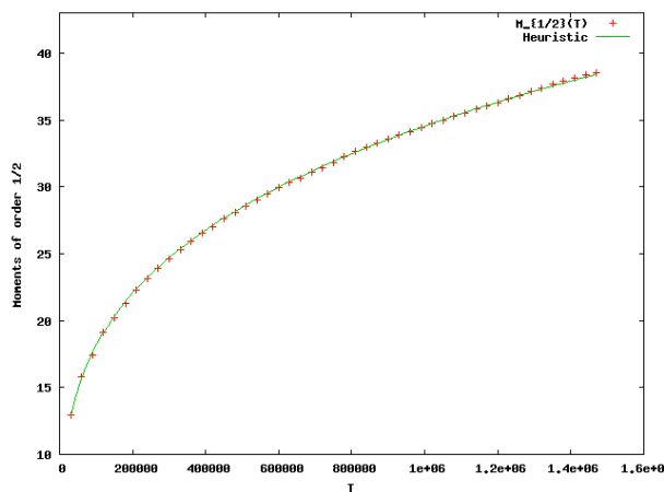
Figure 10: Moments of order \frac{1}{2} and 1 for the regulators of the twists of 17a1 by prime discriminants and the functions given by the heuristics.
