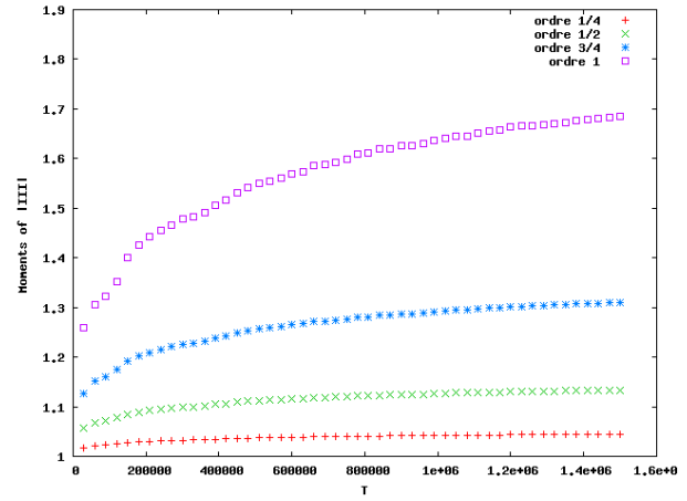
Figure 4: Moments of order \frac{1}{4} , \frac{1}{2} , \frac{3}{4} and 1 for the order of the Tate-Shafarevich groups of the twists of 11a1 . The heuristics suggest that the moments of order k < 1 tend to a constant (depending on k ) whereas the moment of order 1 should tend to infinity.
