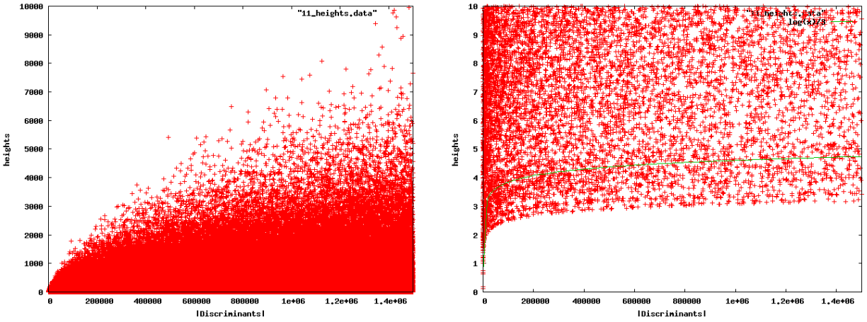
Figure 1: Regulators of the twists of 11a1 . On the left, all the regulators are plotted, and on the right, only regulators less than 10. The gap between the x -axis and the minimal heights is clearly visible on the right.
