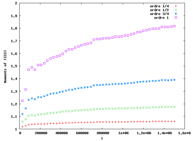
Figure 12: Moments of order \frac{1}{4} , \frac{1}{2} , \frac{3}{4} and 1 of the order of the Tate-Shafarevich groups of the twists of 14a1 . The heuristics suggest that the moments of order k < 1 tend to a constant (depending on k ) whereas the moment of order 1 should tend to infinity.
