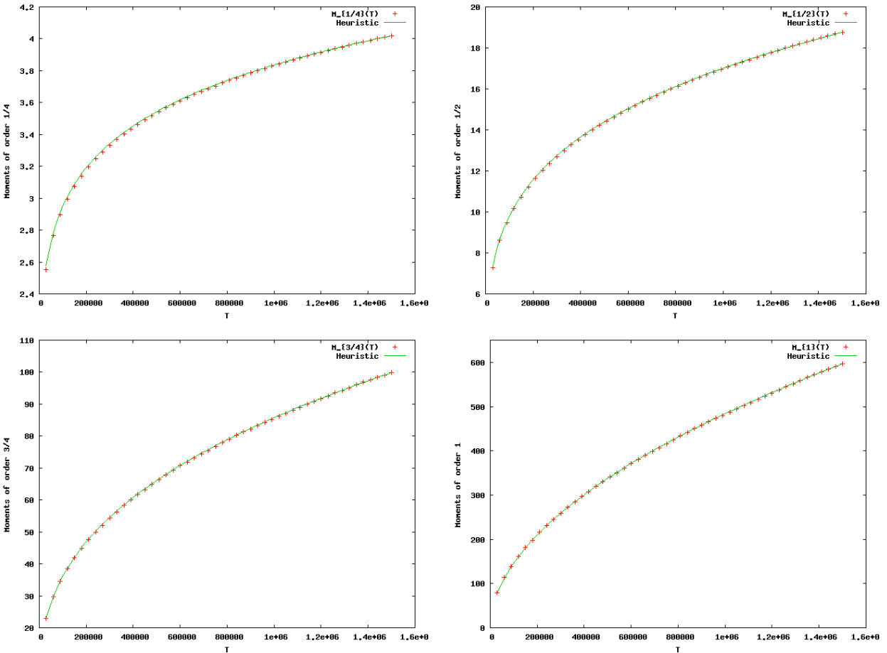
Figure 7: Moments of order \frac{1}{4} , \frac{1}{2} , \frac{3}{4} and 1 of the regulators of the twists of 17a1 and the functions given by the heuristics.
