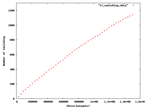
Figure 8: Number of extra-vanishing of L'(E_d, 1) for E = 17a1 .
