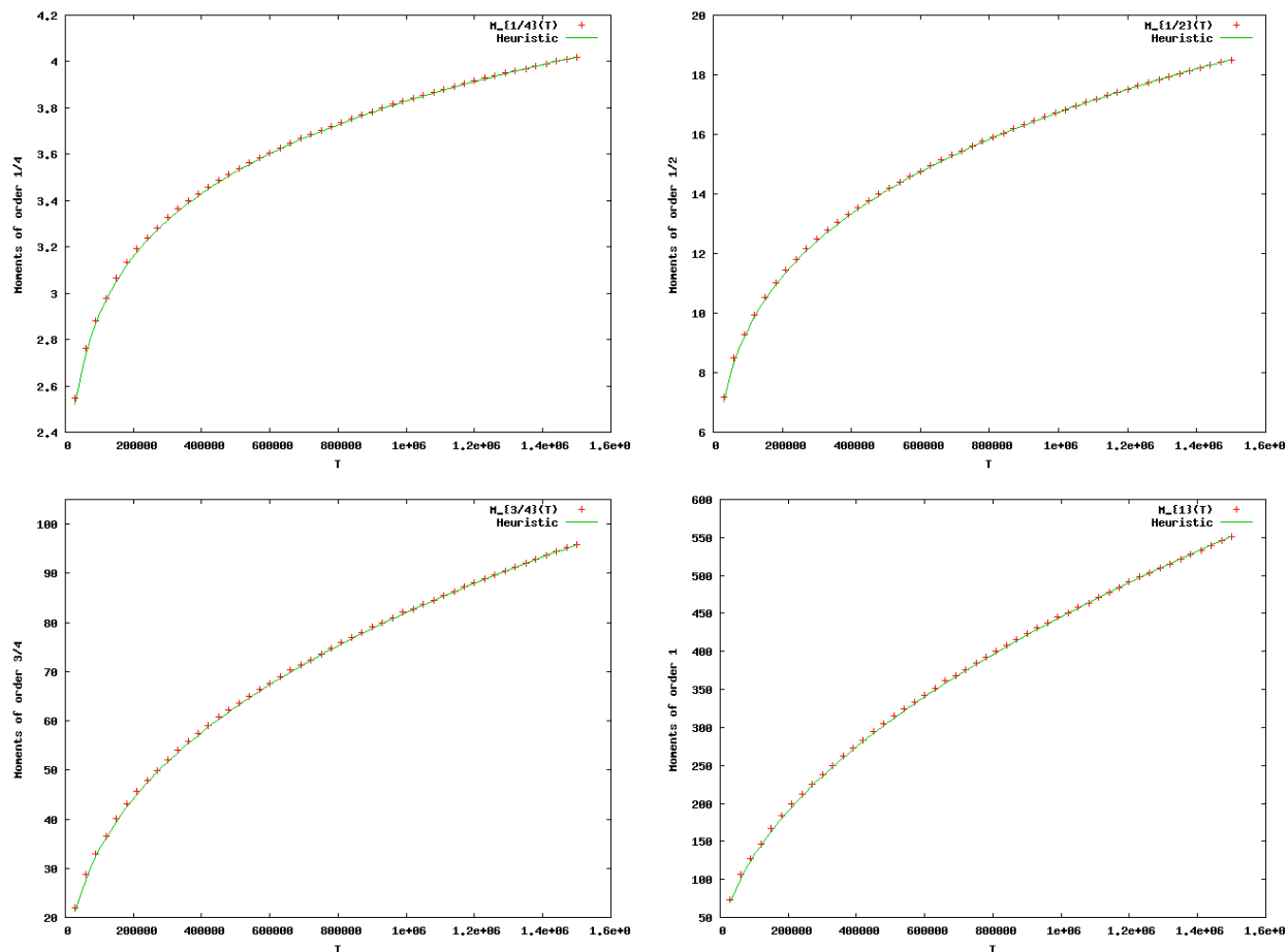
Figure 13: Moments of order \frac{1}{4} , \frac{1}{2} , \frac{3}{4} and 1 of the regulators of the twists of 14a1 and the functions given by the heuristics.
