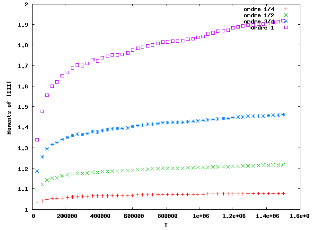
Figure 15: Moments of order \frac{1}{4}, \frac{1}{2}, \frac{3}{4} and 1 of the order of the Tate-Shafarevich groups of the twists of 15a1. The heuristics suggest that the moments of order k < 1 tend to a constant (depending on k ) whereas the moment of order 1 should tend to \infty .
