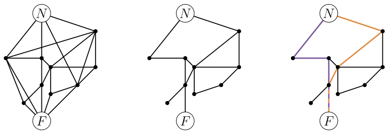
FIG. 2. Second visual aid for the definition of the uniform-geodesic ant process. On the left is pictured a graph \mathcal{G} . In the middle is a possible realization of a graph \mathcal{G}^{(n)} , the trace of the n th random walk. On the right, in orange and purple, are the two geodesics from N to F in \mathcal{G}^{(n)} , and thus the two possible choices for \gamma^{(n)} .
