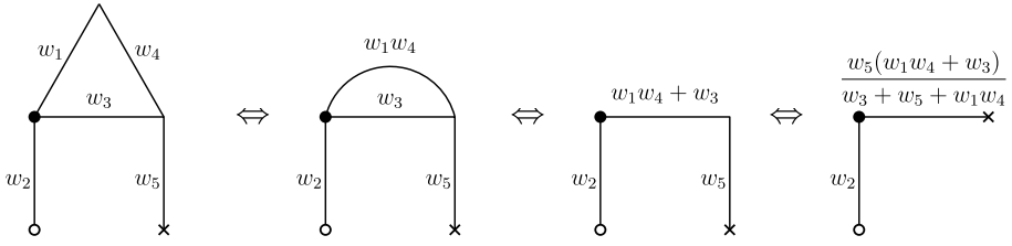
FIG. 9. Calculation of p^\ell(w)/w_1 (i.e. the probability to reach the circled vertex before the crossed vertex starting from the black vertex) for w \in \mathcal{E} (in particular, we use w_1 + w_4 = 1 ).
