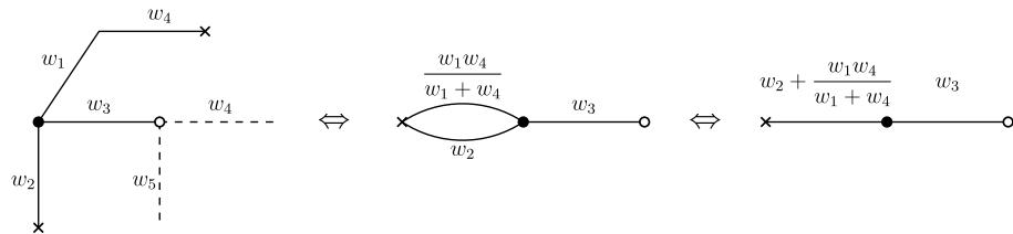
FIG. 7. Calculation of the probability of (ii), the event that a random walker starting at the black dot reaches the white dot before reaching the crosses. The dashed edges in the left-hand side picture have no effect on the calculation and can be removed. In terms of effective conductances between the black dot and the crosses and the black dot and white dot, these three graphs are equivalent.
