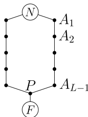
FIG. 11. The graph of Proposition 1.6 and the notation used in Section 4.
