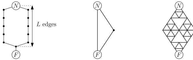
FIG. 5. Graphs used in the discussions of Section 1.3.
