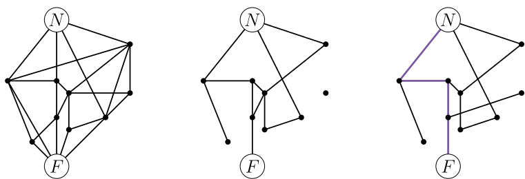
FIG. 1. First visual aid for the definition of the uniform-geodesic ant process. On the left is pictured a graph \mathcal{G} . In the middle is a possible realization of a graph \mathcal{G}^{(n)} , the trace of the n th random walk, and on the right is \gamma^{(n)} the unique geodesic from N to F in \mathcal{G}^{(n)} .
