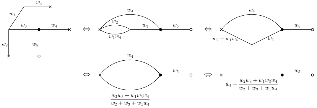
FIG. 8. Calculation of the probability of (iii) in the case w_1 + w_4 = 1 , the event that a random walker starting at the black dot reaches the white dot before reaching the crosses. In terms of effective conductances between the black dot and the crosses and the black dot and white dot, these five graphs are equivalent.
