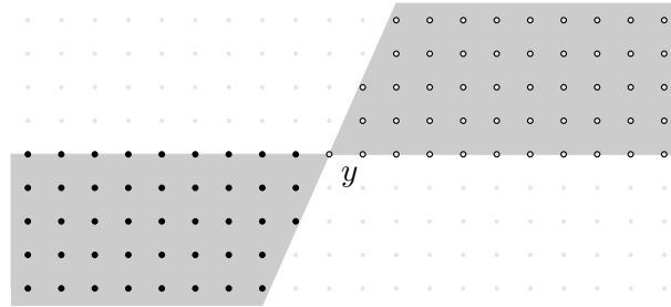
Figure 2: An illustration of the sets \angle(y) (represented by white circles) and \mathcal{T}(y) (represented by filled black circles), with y = (x, n) \in \mathbb{Z}^2 .
