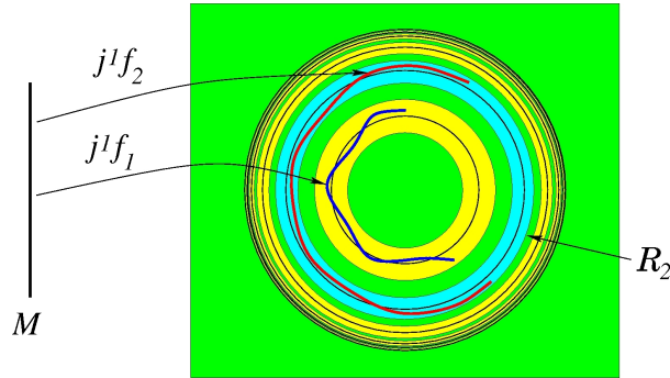
The Gromov machinery is applied iteratively producing a sequence of maps f_1, f_2 , etc.
