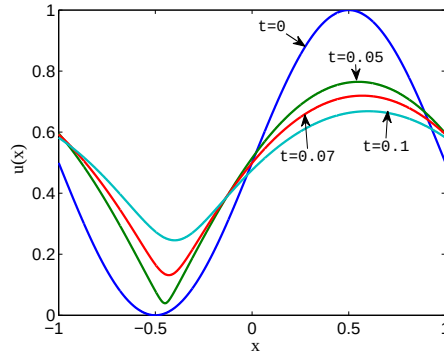
Figure 4.1: Example 1 - Evolution of the approximate solution computed on a fine mesh.
