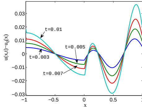
Figure 4.2: Example 2 - Evolution of the deviation from the initial data u(t) - u_0 .
