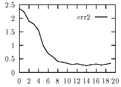
Figure 9: \varepsilon_2 versus iteration
