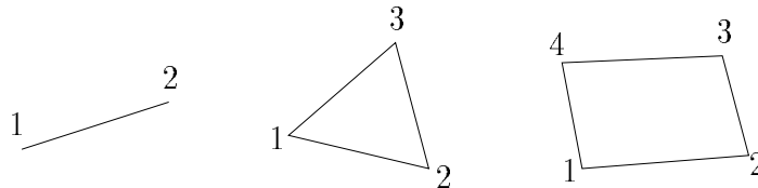
Figure 15: Canonical numbering.
