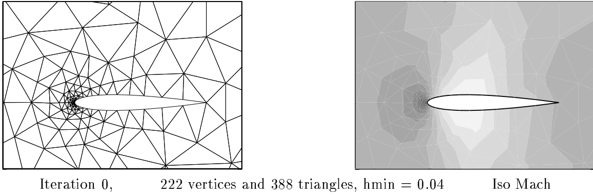
Figure 13: initialisation (Iterations 0)
