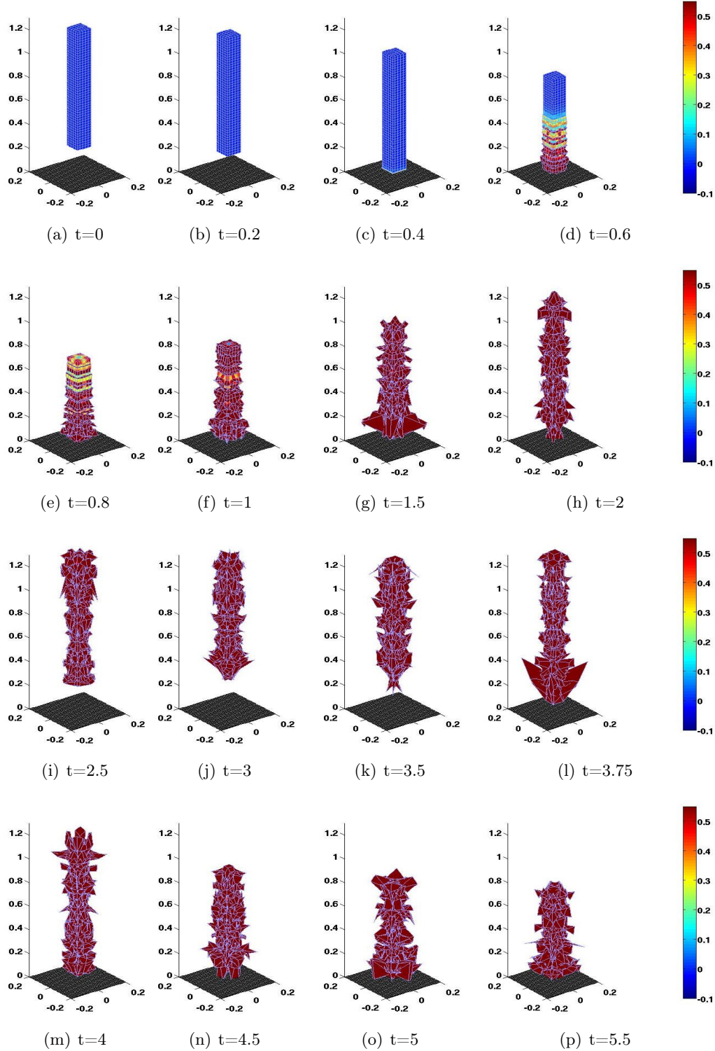
Figure 4.19: Von Mises stress evolution of the deformed bar after the contact by using Crank–Nicolson scheme and with the standard mass matrix ( \Delta \mathbf{x} = 0.02 and \Delta t = 0.01 ).
