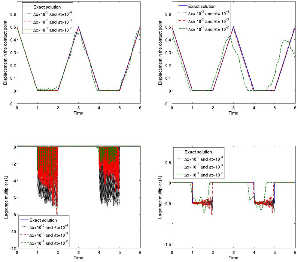
Figure 2.13: Comparison of the analytical solution (u, \lambda) and the approximated solutions (U_h^n, \lambda^n) by using the standard (left) and modified mass matrices (right) in the contact.
