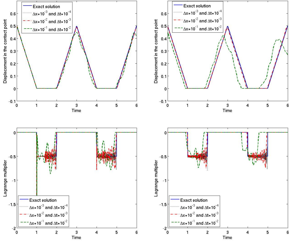
Figure 2.17: Comparison of the analytical solution (u, \lambda) and the approximated solutions (U_h^n, \lambda^n) by using the standard (left) and modified (right) mass matrices in the contact.
