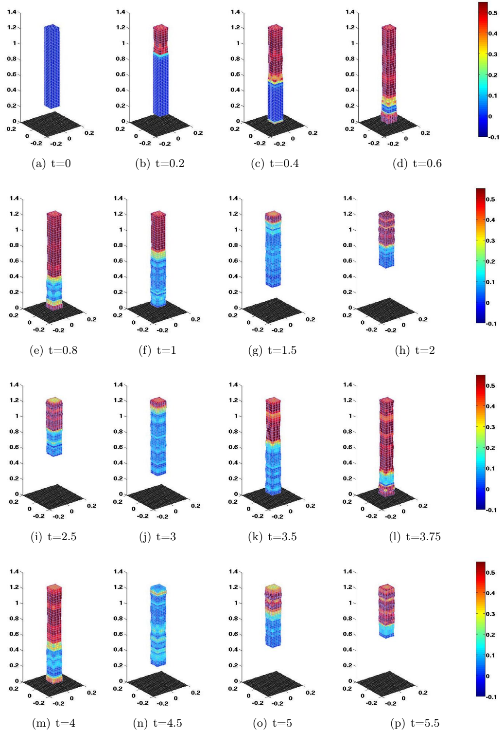
Figure 4.6: Von Mises stress evolution of the deformed bar after the contact by using Crank–Nicolson scheme and with the modified mass matrix ( \Delta \mathbf{x} = 0.02 and \Delta t = 0.01 ).
