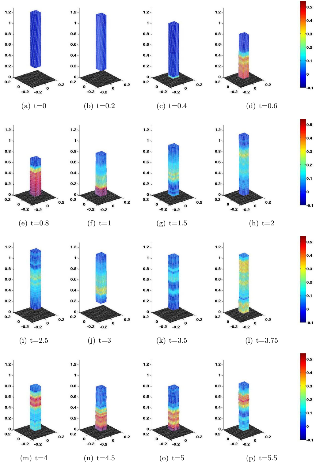
Figure 4.20: Von Mises stress evolution of the deformed bar after the contact by using Crank–Nicolson scheme and with the modified mass matrix ( \Delta \mathbf{x} = 0.02 and \Delta t = 0.01 ).
