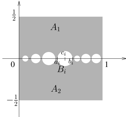
Figure 1: An example illustrating the fact that the M -connected components of an open set do not coincide in general with the classical connected components.
