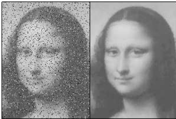
Figure 6: An image corrupted by an impulse noise with frequency 15% and the result of the denoising performed by I_{10}S_{10} .
