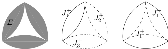
Figure 2: The set E (in grey), its boundaries J^\pm and the boundaries of its complement. The last figure illustrates as well the internal and external boundaries obtained by the topographic function.
