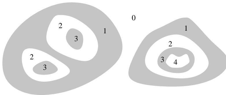
Figure 3: The topographic function associated with the gray set E counts how many boundaries must be crossed to reach the exterior of E .
