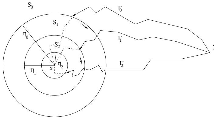
Figure 4: Recursive construction of \Gamma near to x
