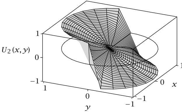
The graph of the harmonic function U_2 along with the boundary of its domain. On the upper-half of unit circle in the xy -plane, this function equals 1; on the lower half of the circle it equals -1 .
