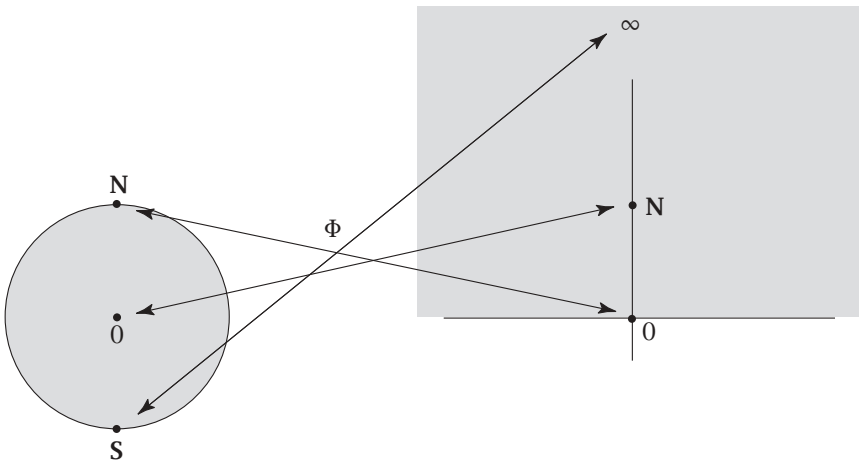
\Phi maps B onto H and H onto B .
