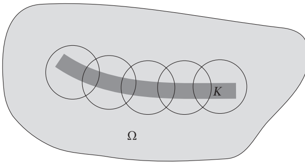
3.7 K covered by overlapping balls.
