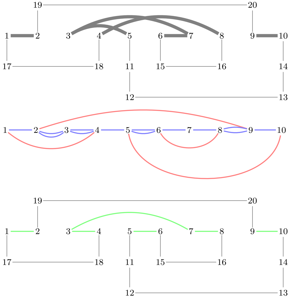
Figure 1: Top: Example of an optimal tour \tau_a with respect to w_a (on |\mathcal{X}| = 20 vertices); thick edges have weight a ( r = 10 here, the space-filling curve visits vertices 1, \dots, 10 in this order). Middle: construction of red and blue edges of \{1, \dots, 10\} . Bottom: an Eulerian circuit visits vertices in this order: 1, 2, 9, 10, 5, 6, 8, 9, 8, 7, 6, 5, 4, 3, 2, 3, 4, 1 . New list of vertices: 1, 2, 9, 10, 5, 6, 8, 7, 3, 4, 1 . In green: not-red edges corresponding to the new list added to the new tour.
