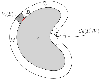
Fig. 3: Offset surface and tube formula. \epsilon -offset of V minus V is
