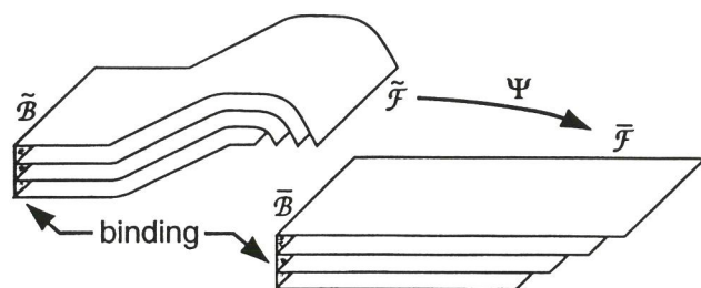
Fig. 2. Unfolding viewed as the transformation \Psi of a folded foliation \tilde{\mathcal{F}} into an unfolded foliation \bar{\mathcal{F}} . The leaves of \bar{\mathcal{F}} should be horizontal. \Psi transforms 'binding surface' \tilde{B} (where leaves cannot slip on each other) to \bar{B} . The binding is shaded.
