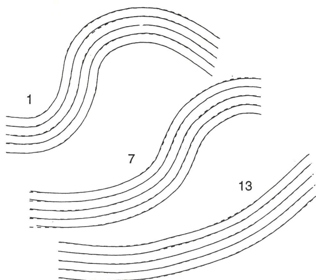
Fig. 16. Digitized cross-sections 1, 7 and 13 (solid lines) and corresponding cross-sections computed from the set of B-spline parameters (dashed lines). Scale: 35% of the original.
