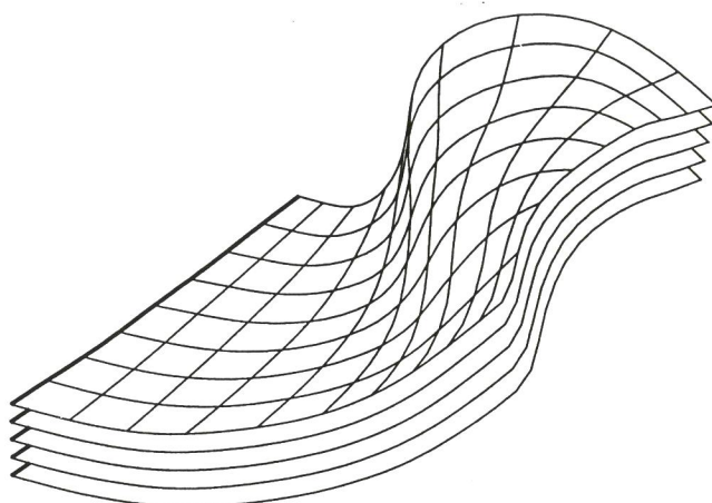
Fig. 17. Perspective view of the folded model. By construction, rear and front faces correspond to cross-sections 1 and 13, hence they are vertical and orthogonal to the binding surface (left face). They do not correspond to original lateral faces.
