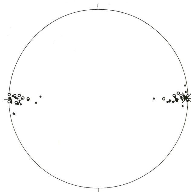
Fig. 19. In this stereographic chart (lower hemisphere projection), dots represent 50 orientations spread out on the face opposite the binding (the right face). The cross represents average value 000.5/89.4W (ideally 000/90). The standard deviation is 9^\circ . Circles represent 17 orientations measured on the same face, obtained with the program UNFOLD.
