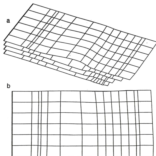
Fig. 15. Same model as in Fig. 13 after unfolding with priority given to volume conservation. (a) Perspective view. (b) Top view.
