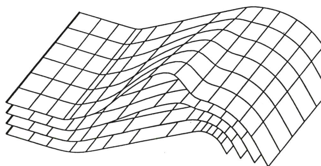
Fig. 13. A folded noncylindrical and nonparallel foliation.
