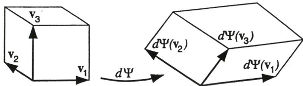
Fig. 5. Volume variation at a point under transformation \Psi , defined as the relative difference between the volume of the parallelepiped spanned by vectors v_1, v_2 and v_3 and the volume of the parallelepiped spanned by vectors d\Psi(v_1), d\Psi(v_2) and d\Psi(v_3) .
