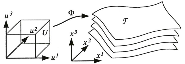
Fig. 6. Parametric representation \Phi maps curvilinear coordinates u^1, u^2 and u^3 into Cartesian coordinates x^1, x^2 and x^3 of points in foliation \mathcal{F} . All points in a leaf in \mathcal{F} have the same value of coordinate u^3 .
