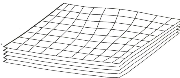
Fig. 18. Model of Fig. 17, after unfolding.
