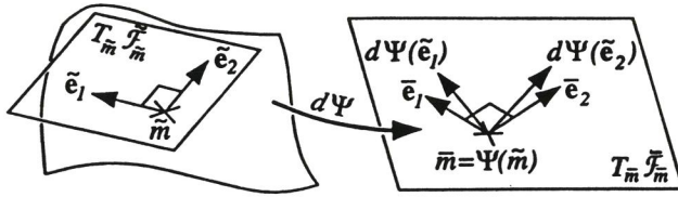
Fig. 4. (\tilde{e}_1(\tilde{m}), \tilde{e}_2(\tilde{m})) is an orthonormal base of plane T_{\tilde{m}} \tilde{\mathcal{F}}_{\tilde{m}} tangent to leaf \tilde{\mathcal{F}}_{\tilde{m}} at \tilde{m} . Similarly, (\bar{e}_1(\bar{m}), \bar{e}_2(\bar{m})) is an orthonormal base of plane T_{\bar{m}} \bar{\mathcal{F}}_{\bar{m}} = d\Psi(T_{\tilde{m}} \tilde{\mathcal{F}}_{\tilde{m}}) tangent to leaf \bar{\mathcal{F}}_{\bar{m}} = \Psi(\tilde{\mathcal{F}}_{\tilde{m}}) at \bar{m} = \Psi(\tilde{m}) . We derive the tangential deformation induced by \Psi from the comparison of bases (d\Psi(\tilde{e}_1), d\Psi(\tilde{e}_2)) and (\bar{e}_1, \bar{e}_2) . Note that we have chosen \bar{e}_1 = d\Psi(\tilde{e}_1)/\|d\Psi(\tilde{e}_1)\| in the text.
