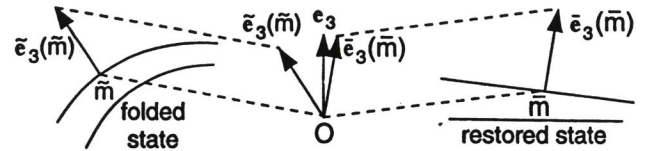
Fig. 3. Unit vector \tilde{\mathbf{e}}_3(\tilde{m}) is normal to the leaves of folded foliation \tilde{\mathcal{F}} , and unit vector \tilde{\mathbf{e}}_3(\tilde{m}) is normal to the leaves of restored foliation \tilde{\mathcal{F}} . Unit vector \mathbf{e}_3 denotes the upward vertical. Unit vectors \tilde{\mathbf{e}}_3(\tilde{m}) or \tilde{\mathbf{e}}_3(\tilde{m}) , which are drawn based at points \tilde{m} or \tilde{m} on the leaf, may be viewed as a mapping, known as the Gauss mapping, from points \tilde{m} or \tilde{m} to points \tilde{\mathbf{e}}_3(\tilde{m}) or \tilde{\mathbf{e}}_3(\tilde{m}) of the unit sphere centred at the origin O.
