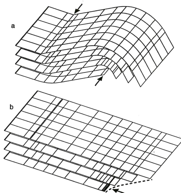
Fig. 10. A thick thrust. (a) Folded structure \tilde{F} . Arrows denote singular lines along which the fold is a chevron . (b) Unfolded structure \tilde{F} . Arrow denotes steeper dips below the ramp.
