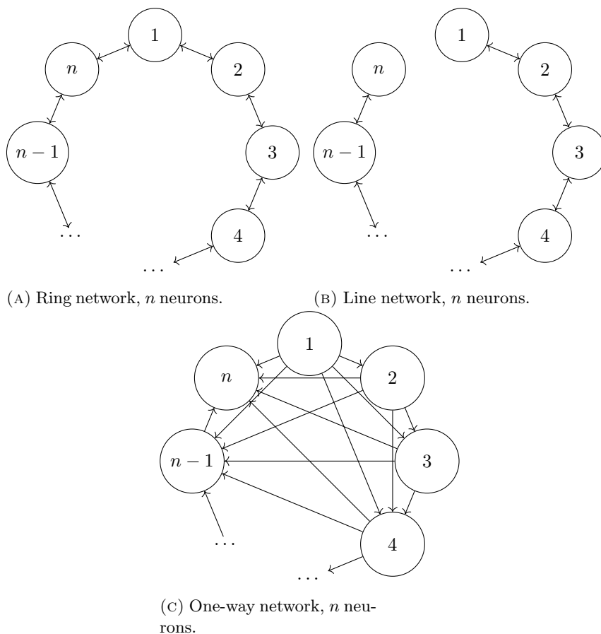
FIGURE 3. The three networks we consider in the sections 3.2, 3.3 and 3.4. We only show the forward case from Section 3.4, as the backward case would look exactly the same but with each arrow reversed.
