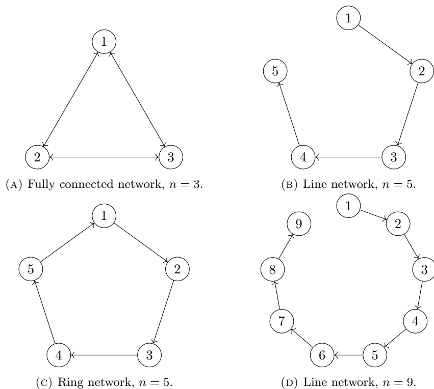
FIGURE 4. The four networks we consider in our numerical simulations. Notice that only the network with n = 3 has double arrows on each edge, representing the fully connected network. The three remaining networks all have unidirectional edges.
