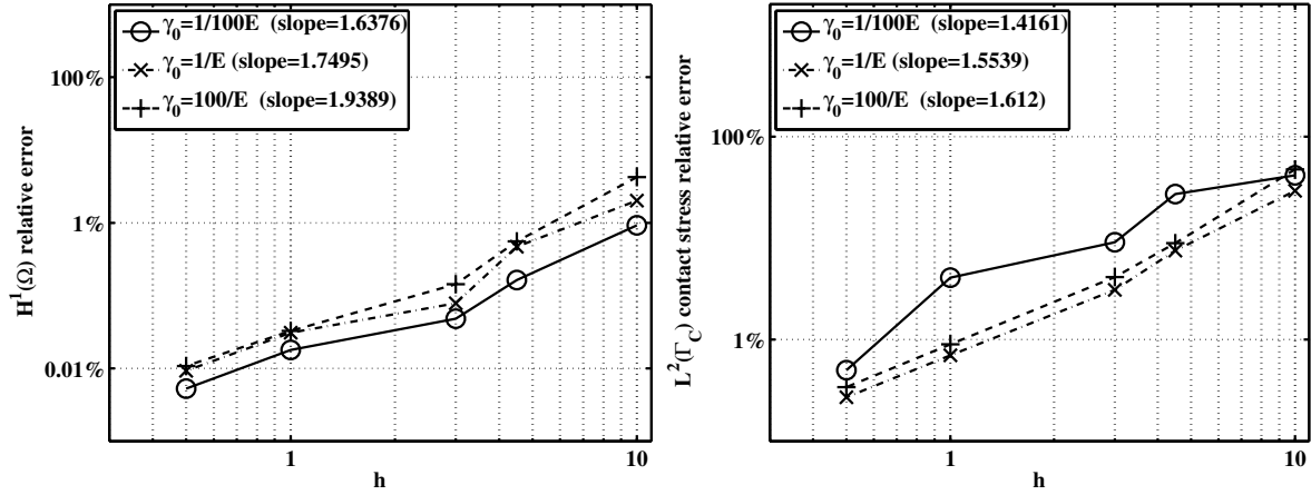
Figure 7: Error curves in the 2D case with P_2 elements and \theta = -1 . Left: relative H^1(\Omega) -norm on the displacements. Right: relative weighted L^2(\Gamma_C) -norm on the contact pressure.
