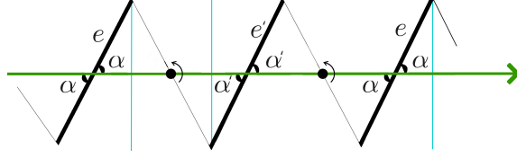
FIGURE 11. Elliptic rotations of even-bipalindromic cutting period-cycles.
