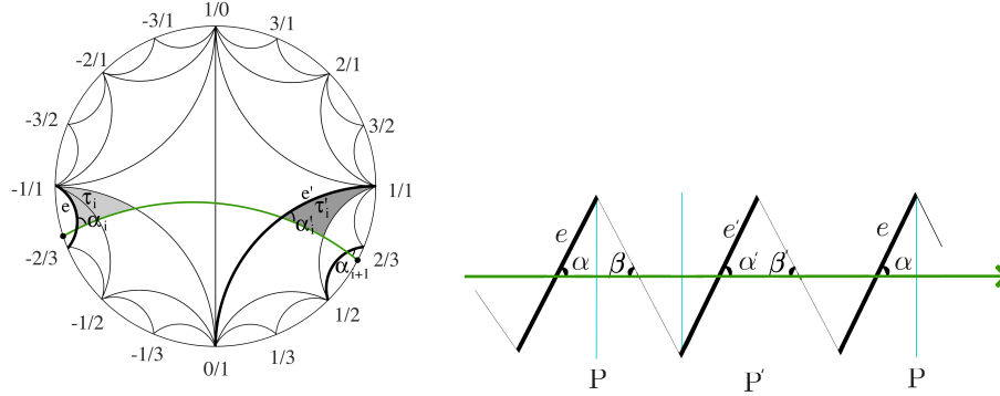
FIGURE 10. Triangles \tau_i and \tau'_i and the interior angles \alpha_i, \alpha'_i, \beta_i, \beta'_i .
