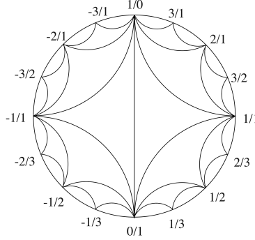
FIGURE 2. Tessellation of \mathbb{D} .
