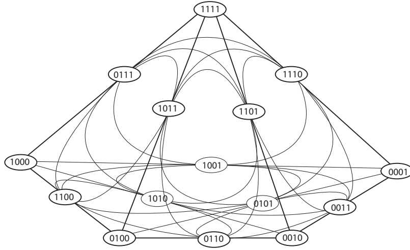
FIGURE 5. The commutation graph of Cl_4 .
