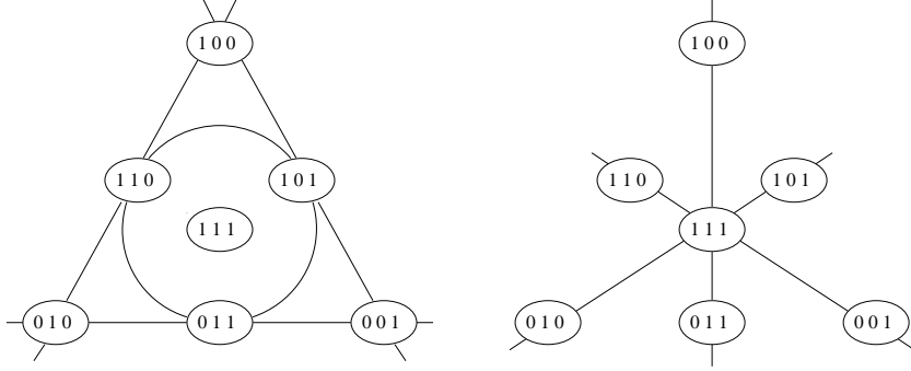
FIGURE 3. The algebras \mathcal{Cl}_3 and \mathbb{M}_3 .
