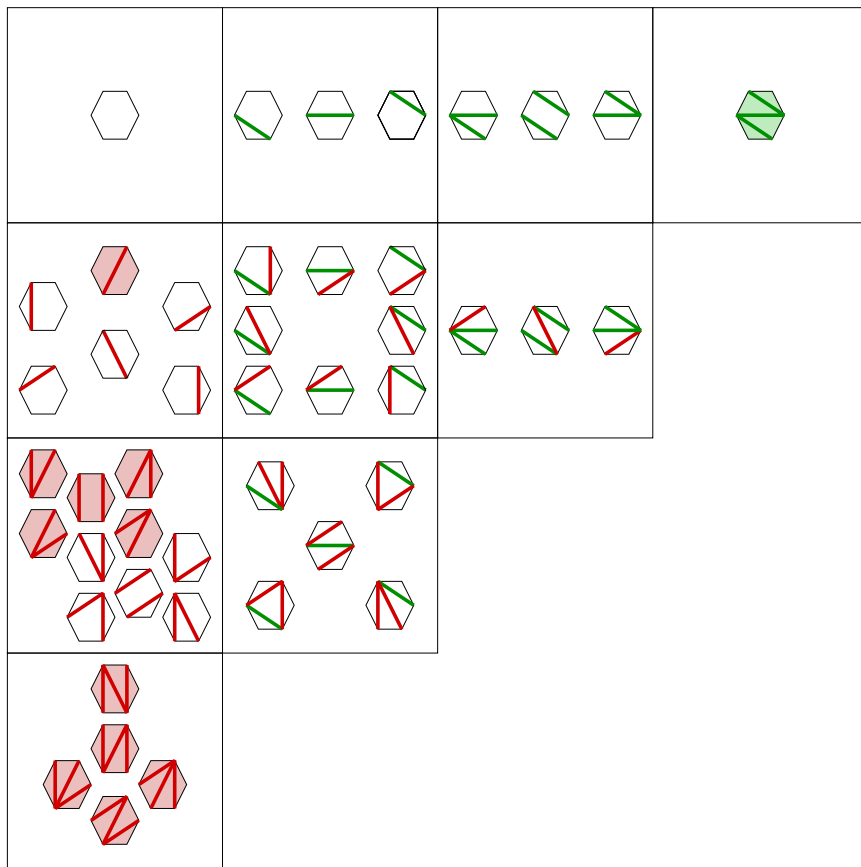
Figure 1: The F -triangle for A_3
