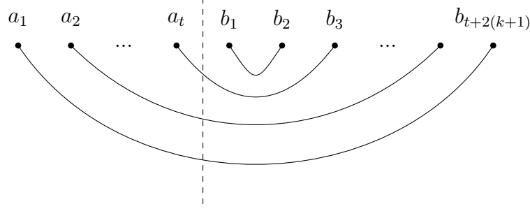
FIGURE 4. Monic diagram t \rightarrow t + 2(k + 1) as a diagram 0 \rightarrow 2t + 2(k + 1) .
